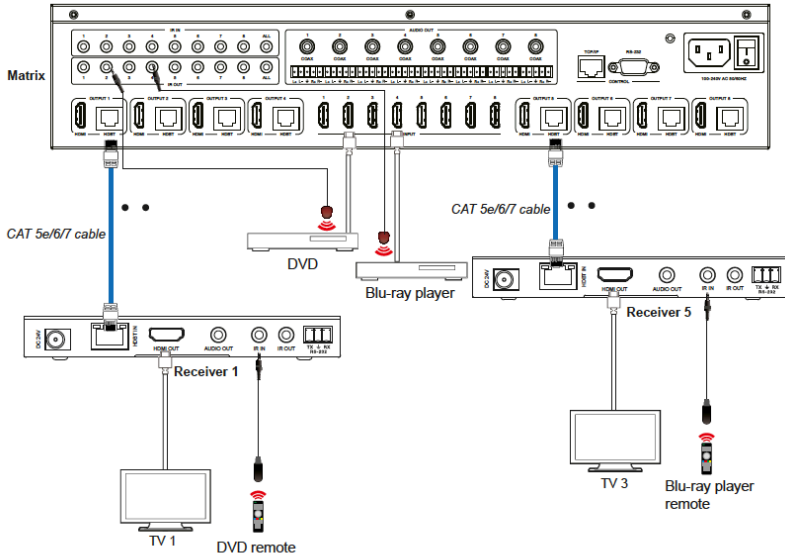
Figure 2: IR connection diagram (HDBaseT Receiver end)
