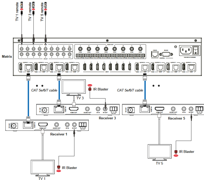
Figure 1: IR connection diagram (Matrix end)
