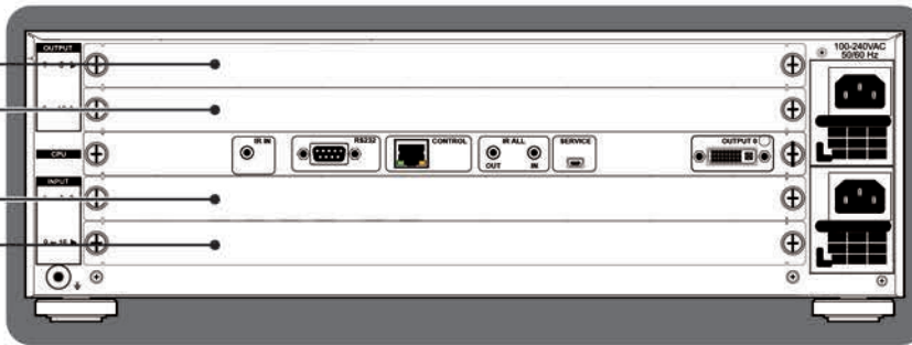
EGE-CDVI-8OUT / 8 Port DVI Output Module
