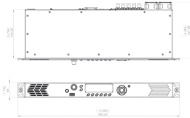
Single Rx 500 rack mount tray with cover (PHRXK1)
