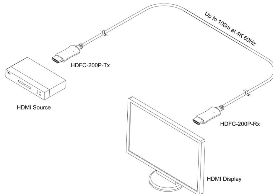
Figure 1 – General connection diagram of HDFC-200P
