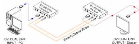
Figure 7 – Connection of 4 LC fiber cables
