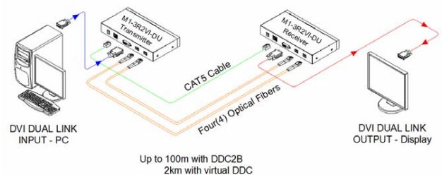
Figure 1 – Overall Optical dual link DVI Module
