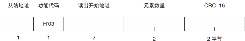
Figure 2-4 Read Out Multiple Registers (0x03)
