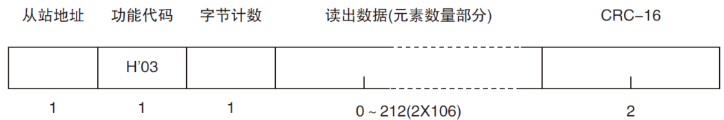
Figure 2-5 Read Out Response Frame of Multiple Registers (0x03)
