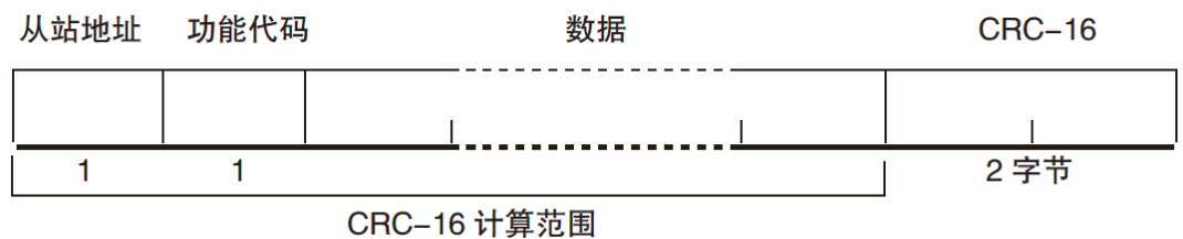
Figure 2-2 Normal Response Frame
