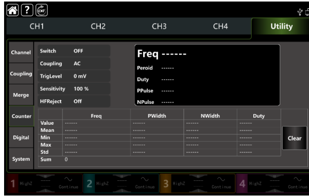
Figure 2-17 Frequency Counter
